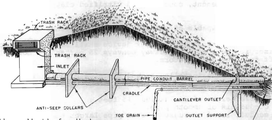
DROP INLET SPILLWAY
