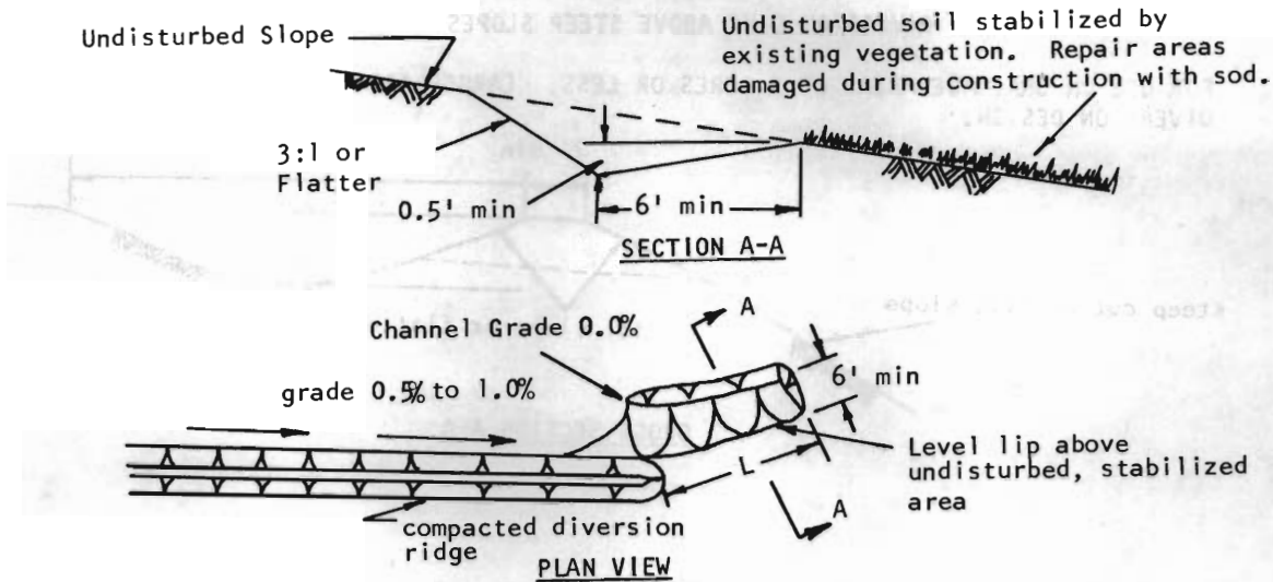
FIGURE 4.2-I LEVEL SPREADER
