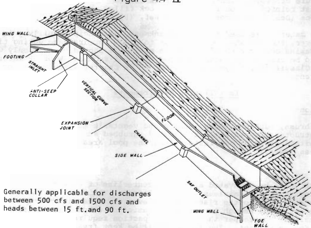
CHUTE SPILLWAY
